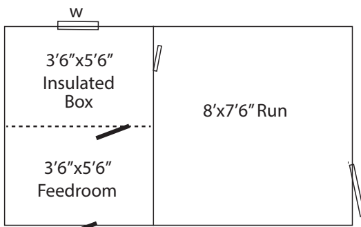
Total Structure Footprint 8x14
