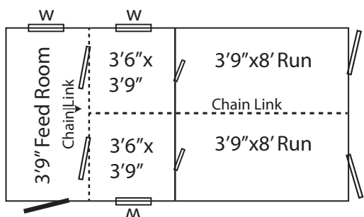
Total Structure Footprint 8x16
